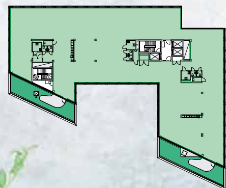
Plan 9: 1 072 m 2
